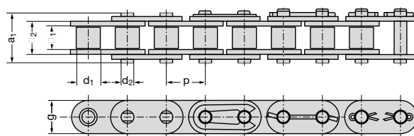
B inner link A outer link E connecting link with spring clip G connecting link with single wire S connecting link with cotter pin
